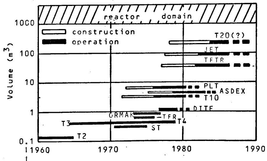
C - PLASMA VOLUME IN TOKAMAKS.
