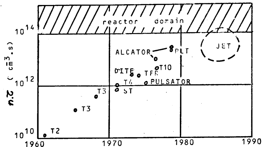
A - QUALITY OF CONFINEMENT IN TOKAMAKS.
